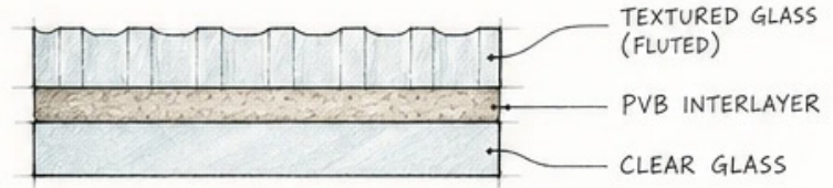
SECTION (SANDWICHED GLASS)
